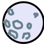
The Moon
