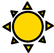
The Sun
