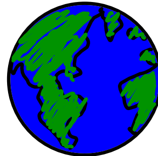
The Earth
